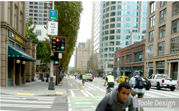
Toole Design Reflective back plate makes the signal more visible
