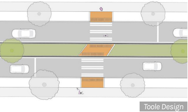
Typical crossing island
