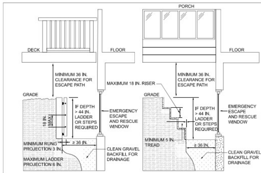
Commentary Figure R310.4.2 LADDERS AND STEPS
