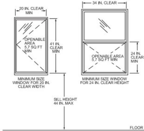
Commentary Figure R310.2.1 EMERGENCY ESCAPE AND RESCUE WINDOW
