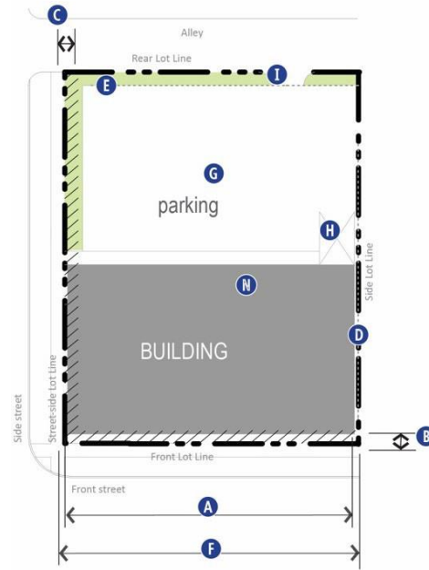
Building Siting.
