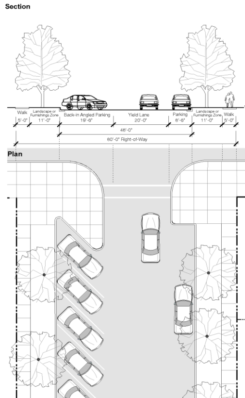
Figure 27-906(7a). Typical Sample Neighborhood Street.
