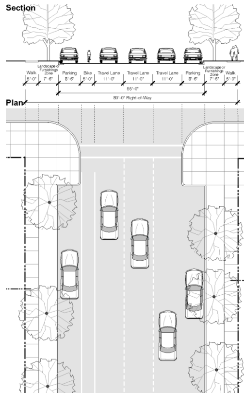
Figure 27-906(10a): Typical Sample One-Way Boulevard - 6th Ave N & Portions of 1st Ave N
