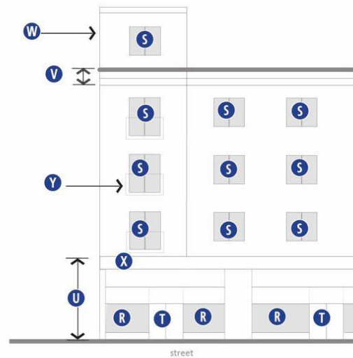
Figure 27-904(13): Building Siting.
