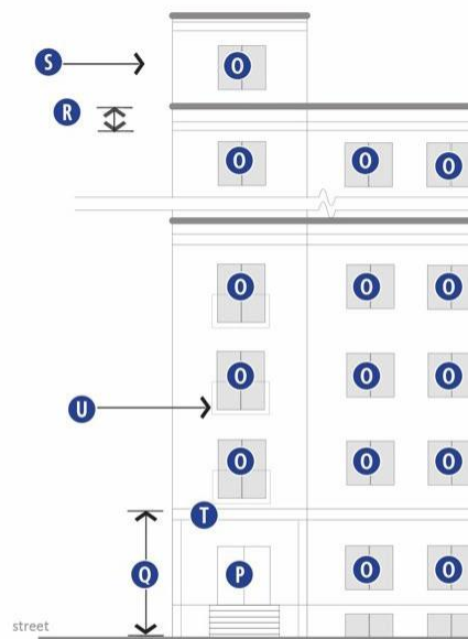
Street Facade Requirements.
