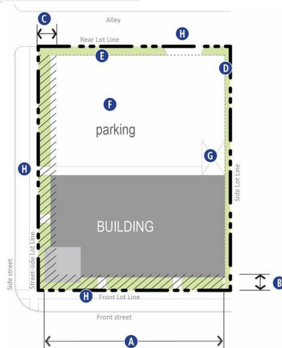
Building Siting.
