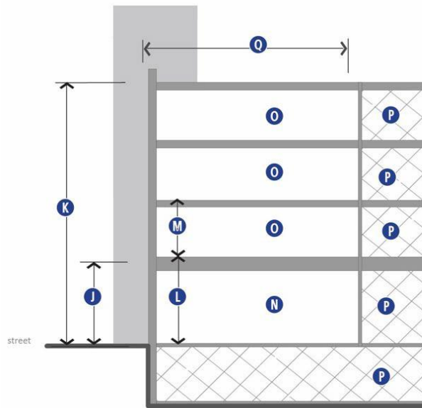
Figure 27-904(14): Height &amp; Use Requirements
