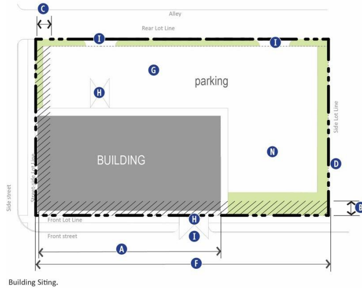
Figure 27-904(10): Building Siting.
