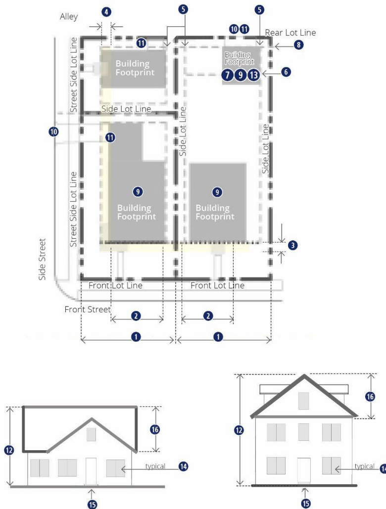
Figure 27-300(1). N1 district diagrammatic plans and elevations.
