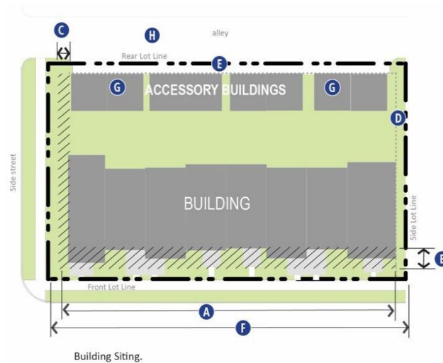
Figure 27-904(1): Building Siting.
